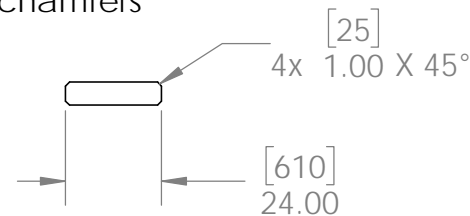
2x6 Cedar Board 2 scab support with chamfers
